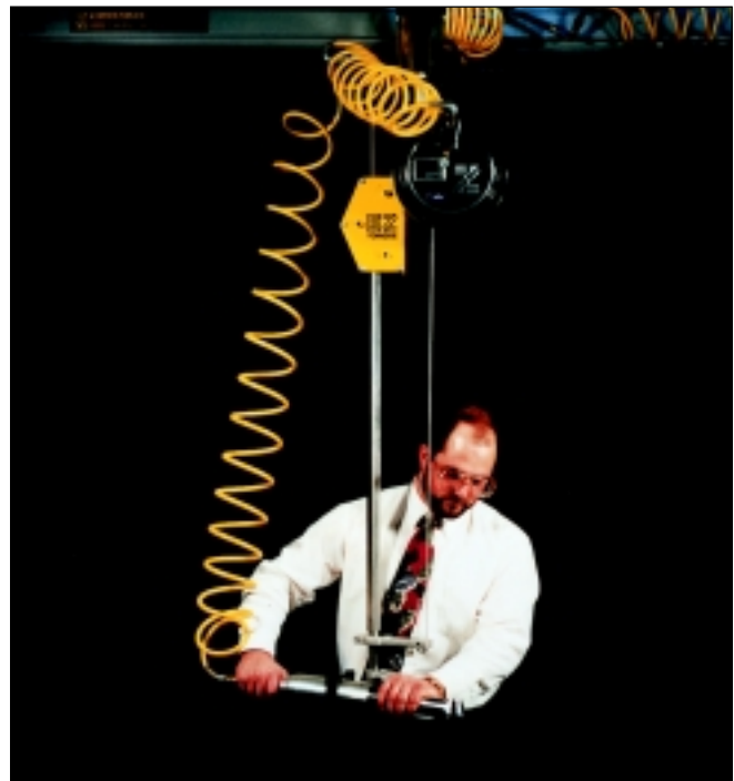
E-Z Torque shown with optional tool
