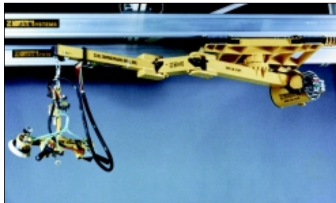
700 C Arm (carriage mount) shown with optional end effector
